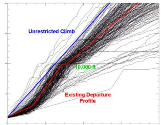
Figure 5: Climb Profiles out of ATL
