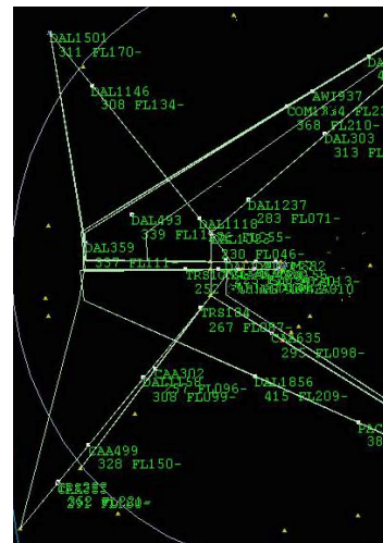
Figure 6: CDAs into ATL direct from IAF to Base-Leg
